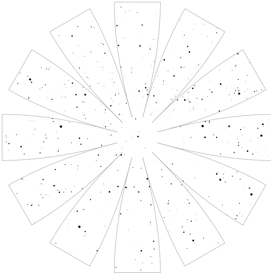
The Northern Hemisphere of Stars
