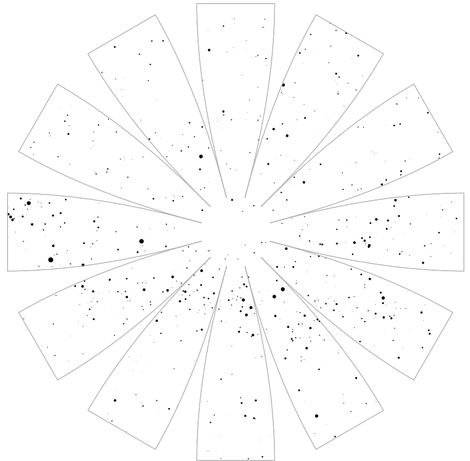
The Southern Hemisphere of Stars
