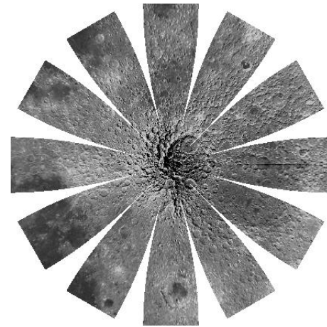
Southern Hemisphere
