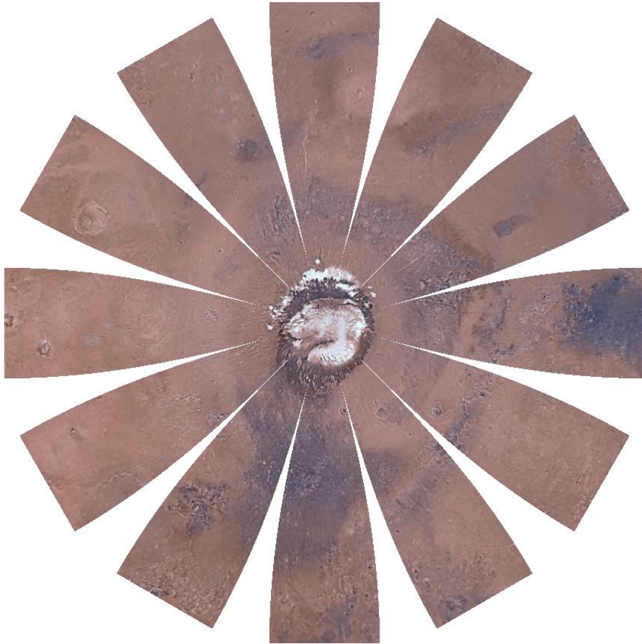
Northern Hemisphere
