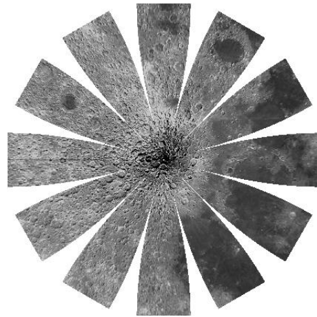
Northern Hemisphere
