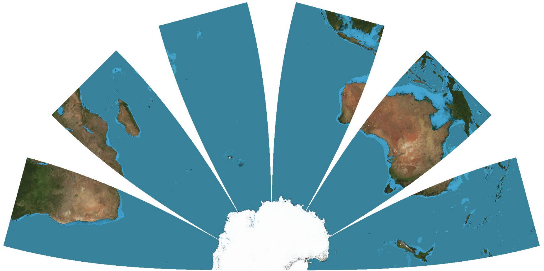
Southeastern Quarter-Sphere
